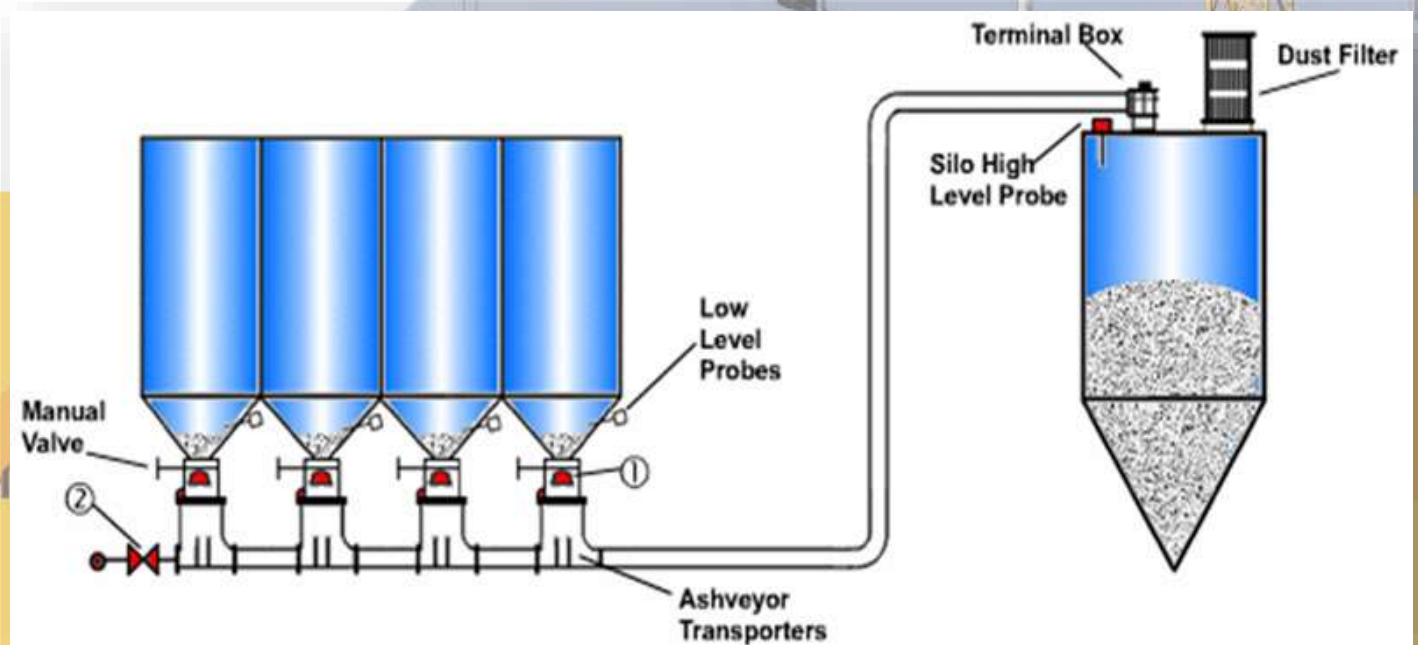
PNEUMATIC ASH HANDLING SYSTEM
